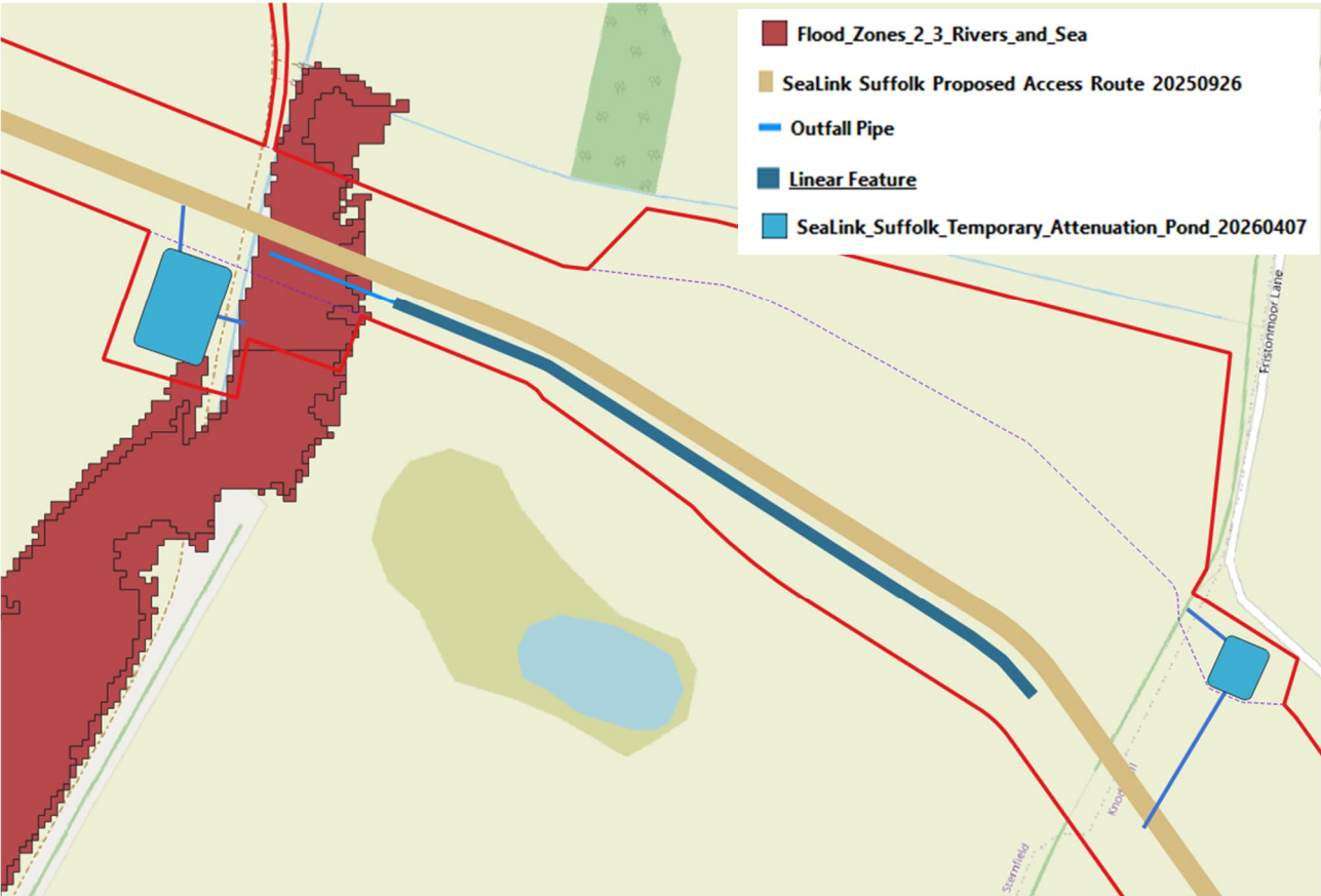
Figure 1 – Illustrative drainage layout
